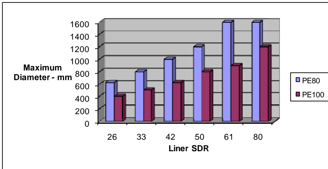
Figure 3-14. Relationship Between Diameter and SDR for Folding
